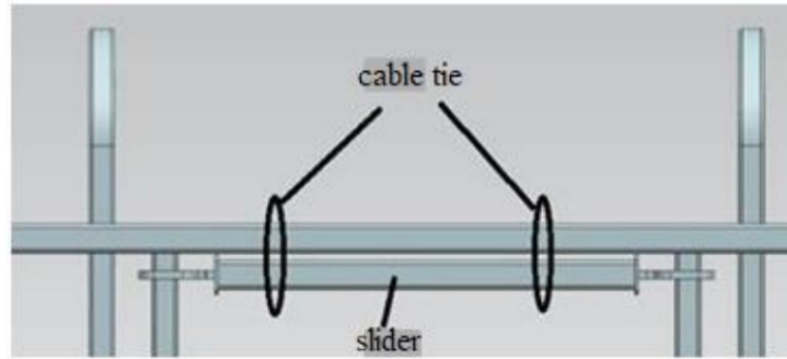
Figura 4-7 Securizarea platformei
